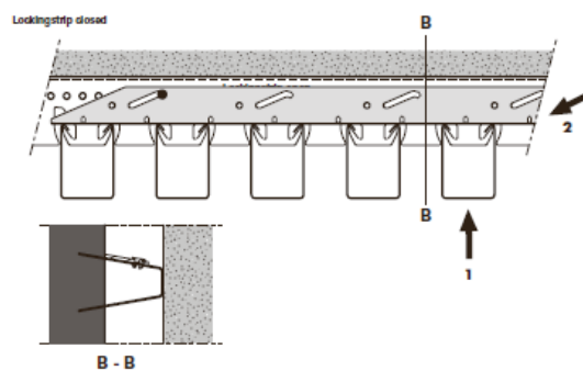
HeartFelt® Wall locking strip
