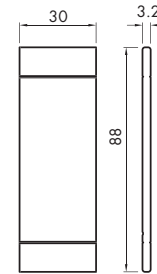
spacer 88 mm
