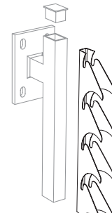
Stringer & rectangular hollow section (in combination with washer sets)
