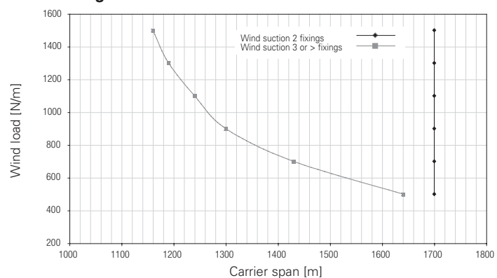
Design chart of carrier V100
