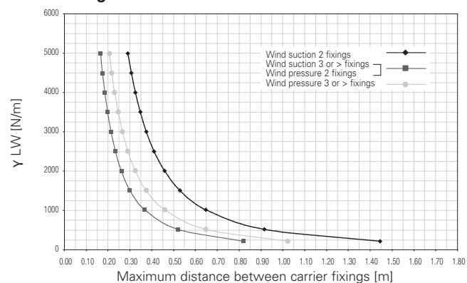
Design chart of carrier 84C
