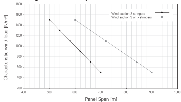
Design chart of V100 panel
