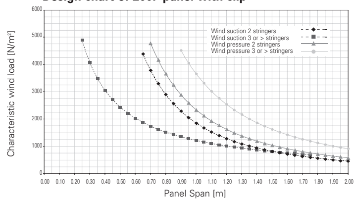
Design chart of 200F panel with clip
