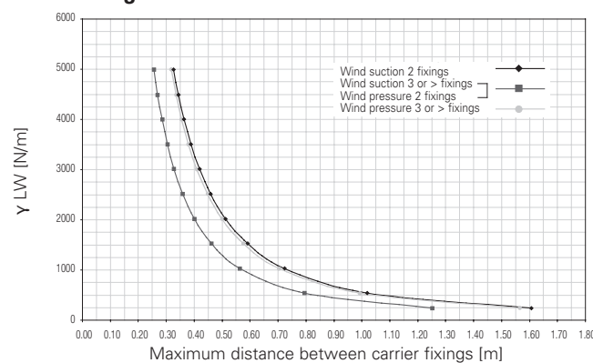
Design chart of carrier 80B
