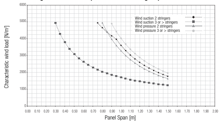
Design chart of 70U panel with locking clip
