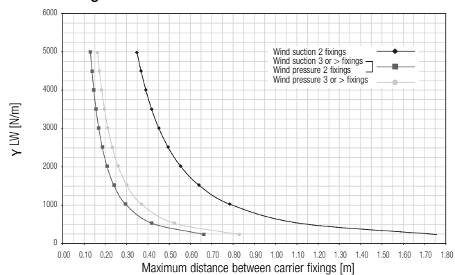
Design chart of carrier 185U
