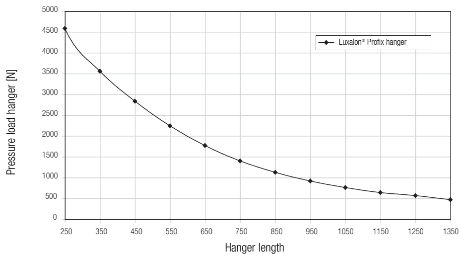
Buckling Luxalon® Profix hanger
