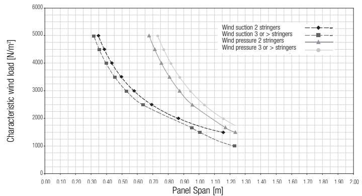
Panel spans 75C
