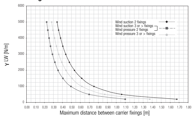
Design chart of carrier 84B
