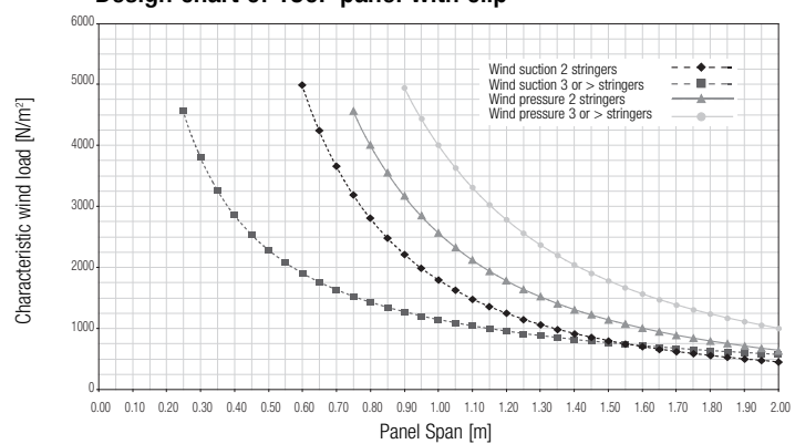
Design chart of 150F panel with clip
