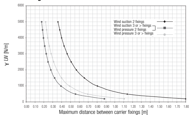
Design chart of carrier 150F
