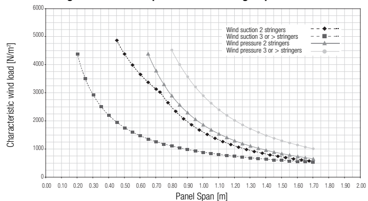
Design chart of 84R panel with locking clip
