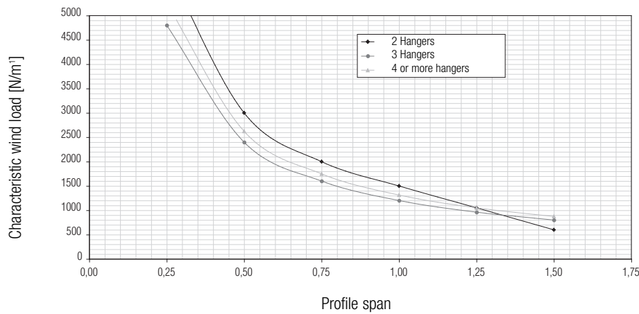
Spantable Luxalon® Profix Profile
