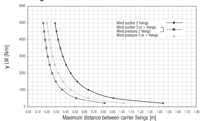
Design chart of carrier 84C
