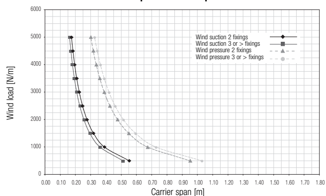
75C-225C Carrier spans closed panels
