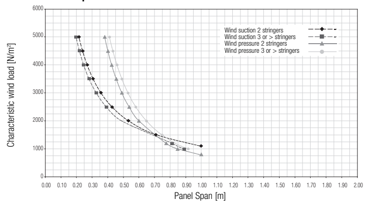
Panel spans 225C
