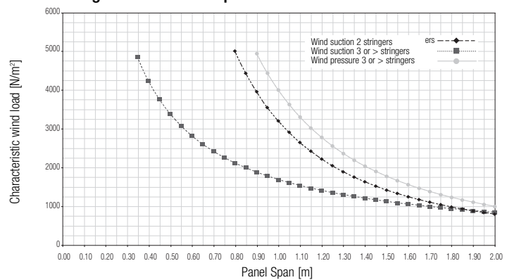
Design chart for 185U panel
