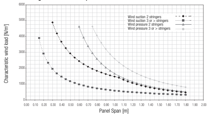
Design chart of 84C panel
