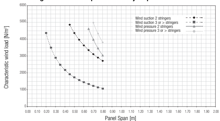
Design chart of 84R panel with U-join profile
