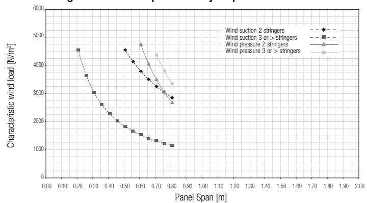
Design chart of 80B panel with join profile
