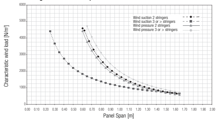
Design chart of 84B panel
