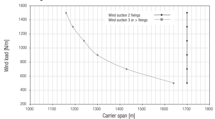
Design chart of carrier V100
