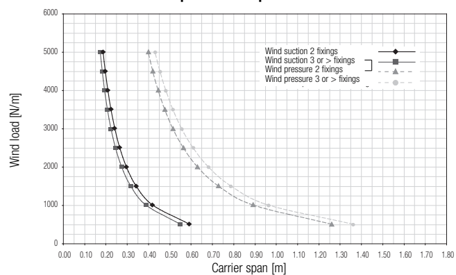
300ACL Carrier spans wide panel
