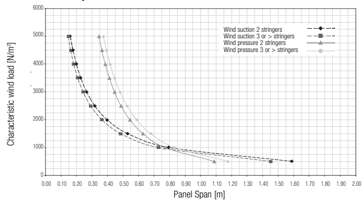
Panel spans 300A
