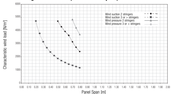
Design chart of 84R panel with V5-join profile
