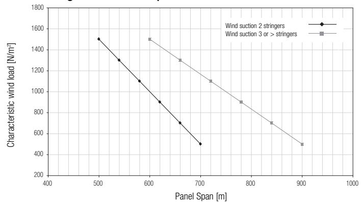
Design chart of V100 panel
