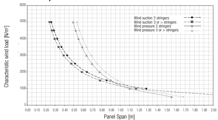
Panel spans 300C/300L
