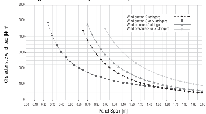
Design chart of 200F panel with clip
