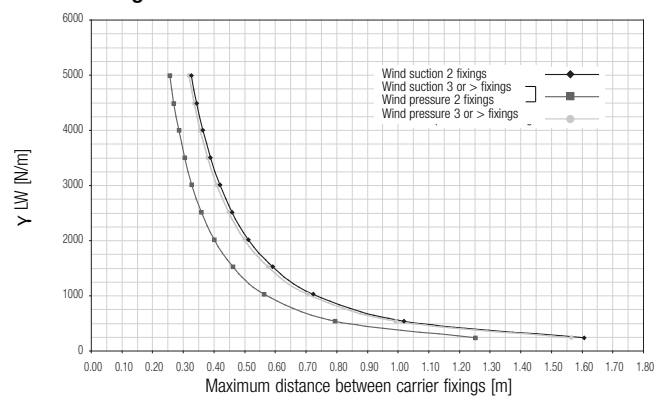
Design chart of carrier 80B
