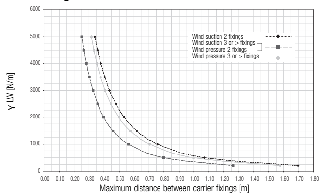
Design chart of carrier 70U
