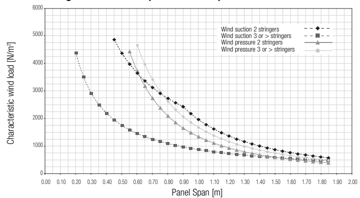
Design chart of 80B panel with clip
