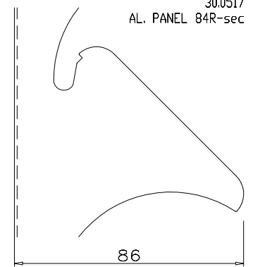
30.1444 SL-STRINGER 4-side
