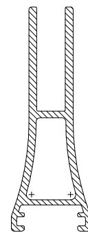
30.4604 SLR 60V-sec
