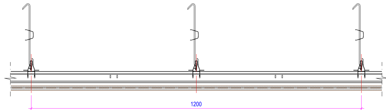
CROSS-SECTION 1 scale 1:8
