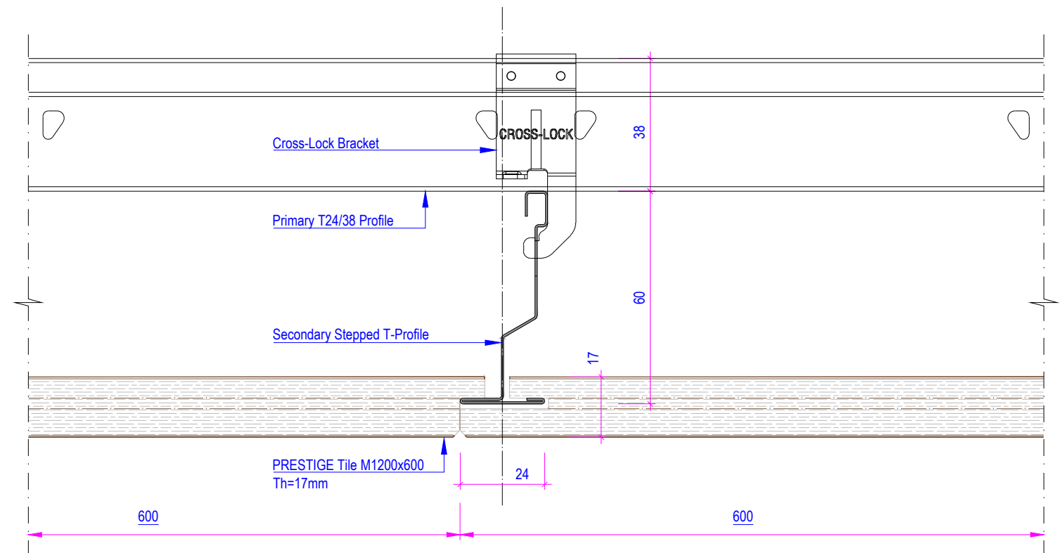
DETAIL SECTION 2 scale 1:1,5
