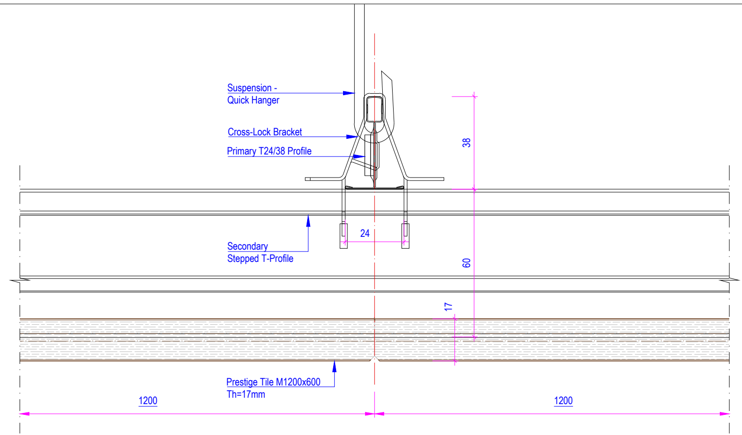
DETAIL SECTION 1 scale 1:1,5
