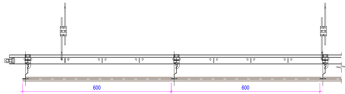
CROSS-SECTION 2 scale 1:8
