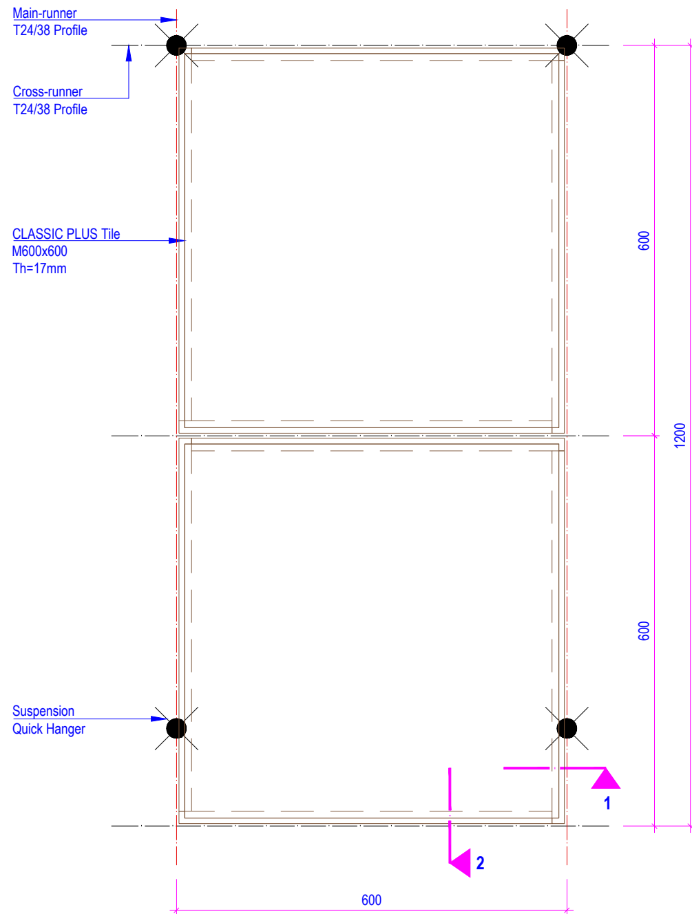
TOP VIEW scale 1:8
