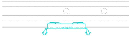
RAIL MOD.135mm. (FOR MOVABLE PANEL) -side
