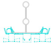
RAIL (FOR MOVABLE PANEL) -front
