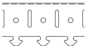
33.9461 AL CARRIER 75C/150C/225C-side
