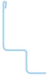
33.2424 EDGE PROFILE 0.8 AL-W 45x21x21x18.5-sec
