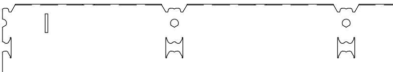
33.7003 MAIN RUNNER C40 MOD.100-side
