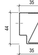
EDGE-PROFILE UW 40 L= max.3000 mm
