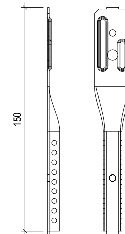
Side view 150 Front view 13
