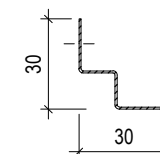
EDGE-PROFILE W 30 L= max.3000 mm
