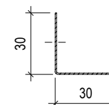
EDGE-PROFILE L 30 L= max.3000 mm
