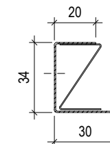
EDGE-PROFILE U 30 L= max.3000 mm
