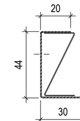
EDGE-PROFILE U 40 L= max.3000 mm
