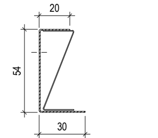
EDGE-PROFILE U 50 L= max.3000 mm
