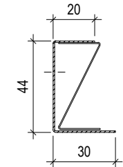
EDGE-PROFILE U 40 L= max.3000 mm
