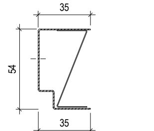
EDGE-PROFILE UW 50 L= max.3000 mm
