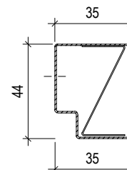
EDGE-PROFILE UW 40 L= max.3000 mm
