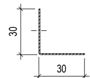
EDGE-PROFILE L 30 L= max.3000 mm
