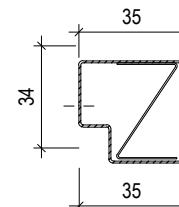
EDGE-PROFILE UW 30 L= max.3000 mm
