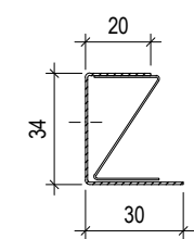
EDGE-PROFILE U 30 L= max.3000 mm
