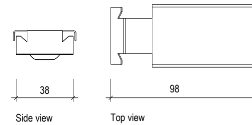
Tavola LOCKING CLIP AL/FE 40TB
