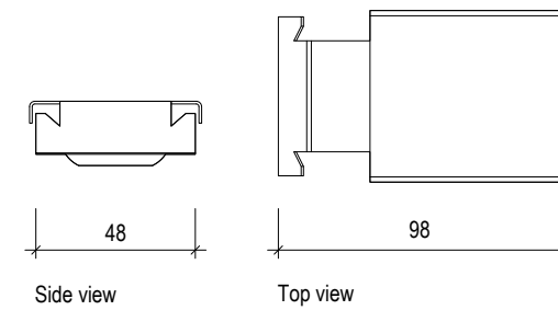
Tavola LOCKING CLIP AL/FE 50TB
