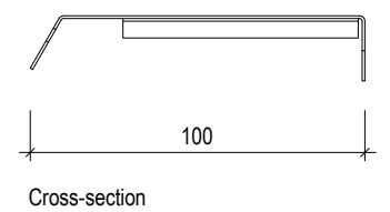
Cross-section Tavola LOCKING CLIP AL/FE 30TB-50TB
